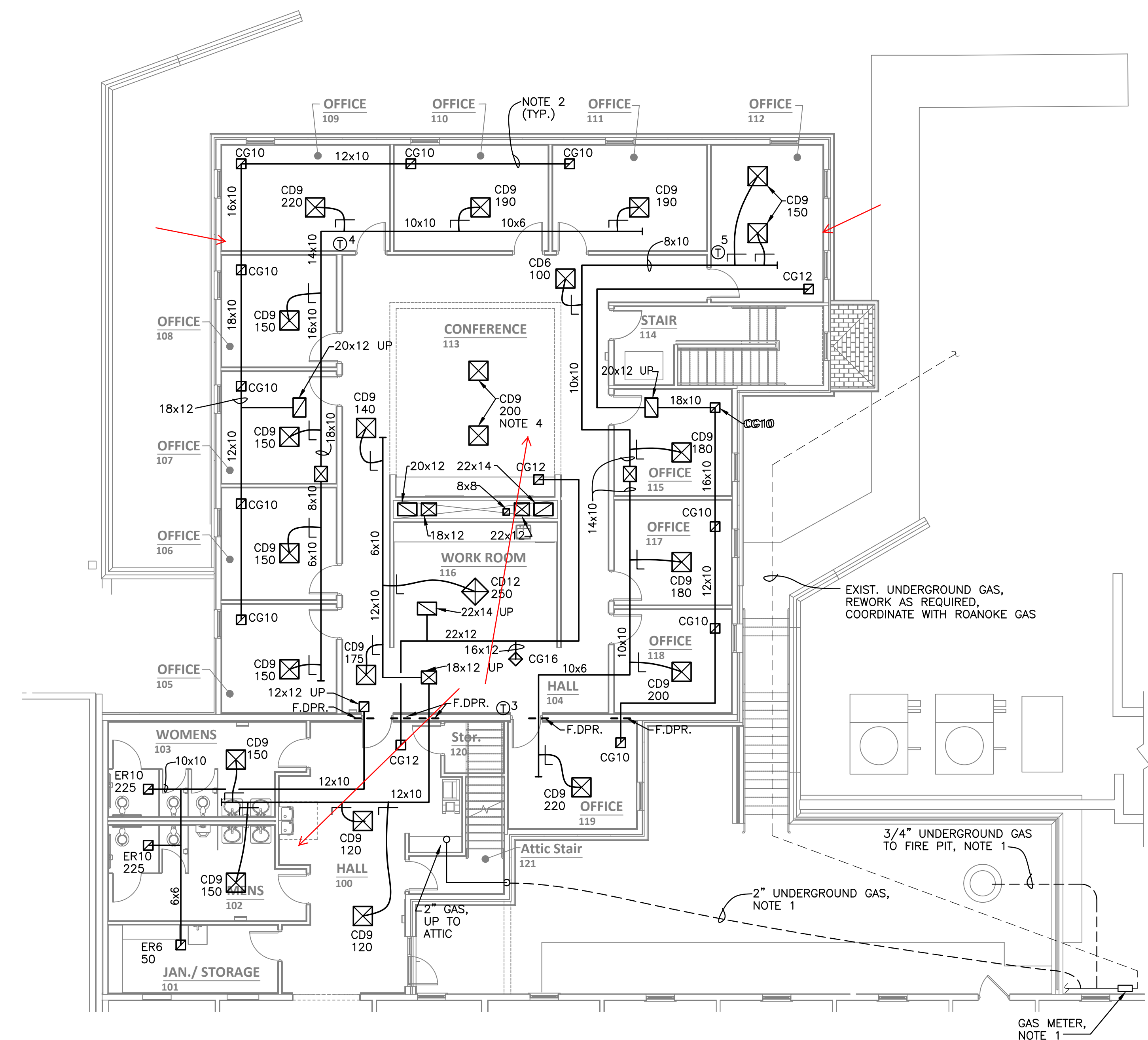
FIRST FLOOR PLAN - MECHANICAL NEW WORK SCALE: 1/8"=1'-0"
