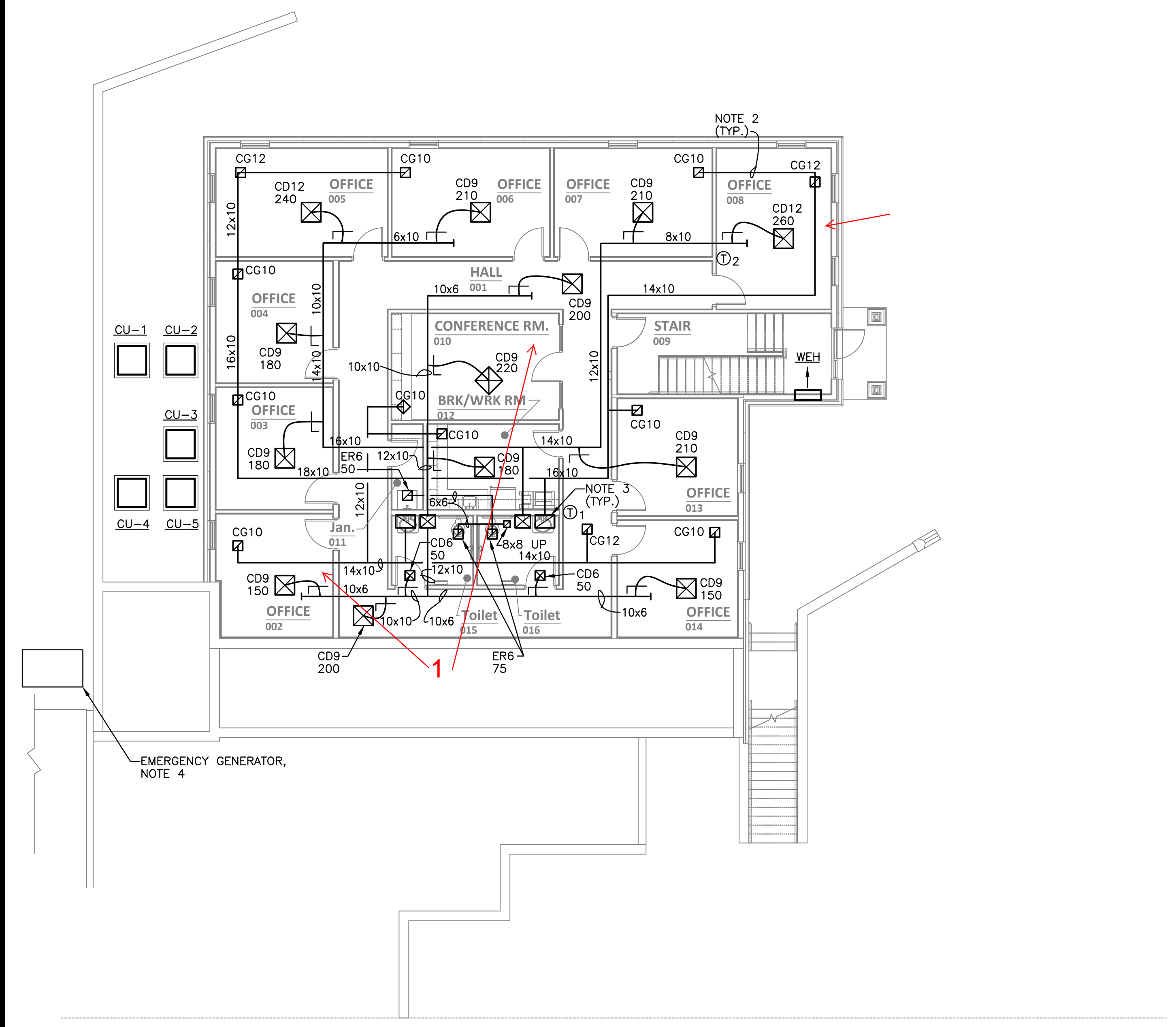
GROUND FLOOR PLAN - MECHANICAL NEW WORK SCALE: 1/8"=1'-0"
